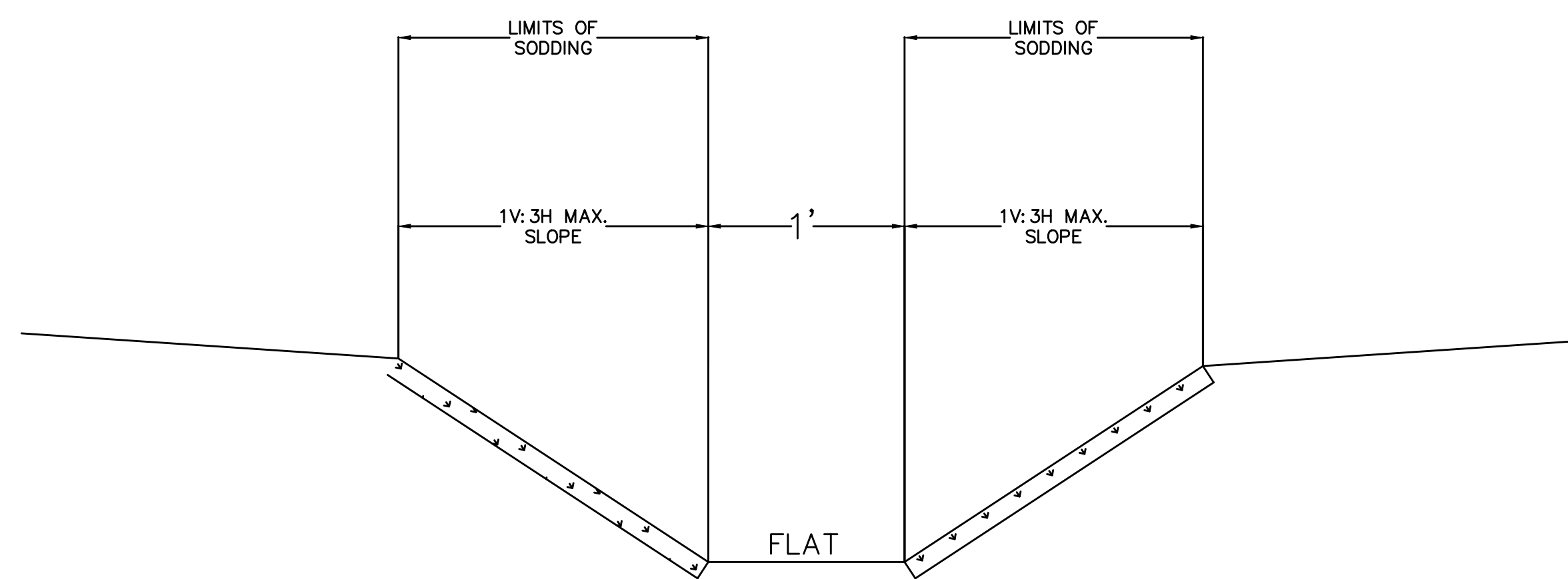
TYPICAL DITCH SECTION
